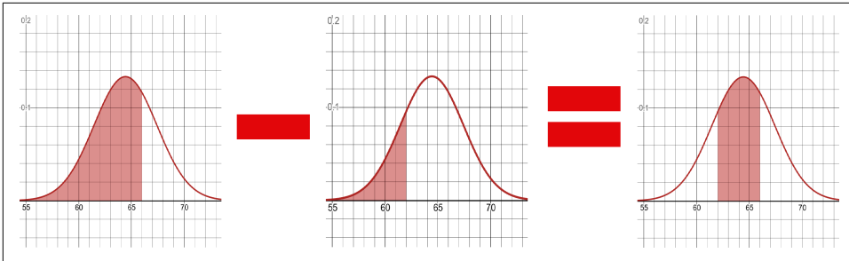
Figure 3-10. Finding a middle range of probability
