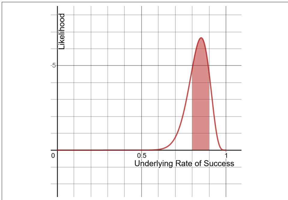
Figure 2-8. Probability the underlying rate of success is between 80% and 90%
