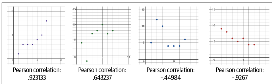
Figure 5-12. Correlation coefficients for four scatterplots
